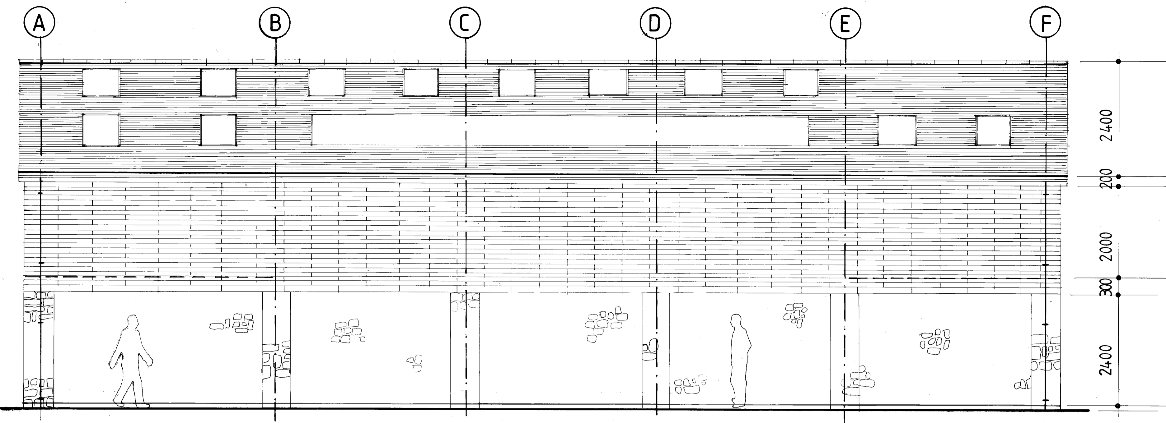
WEST ELEVATION
