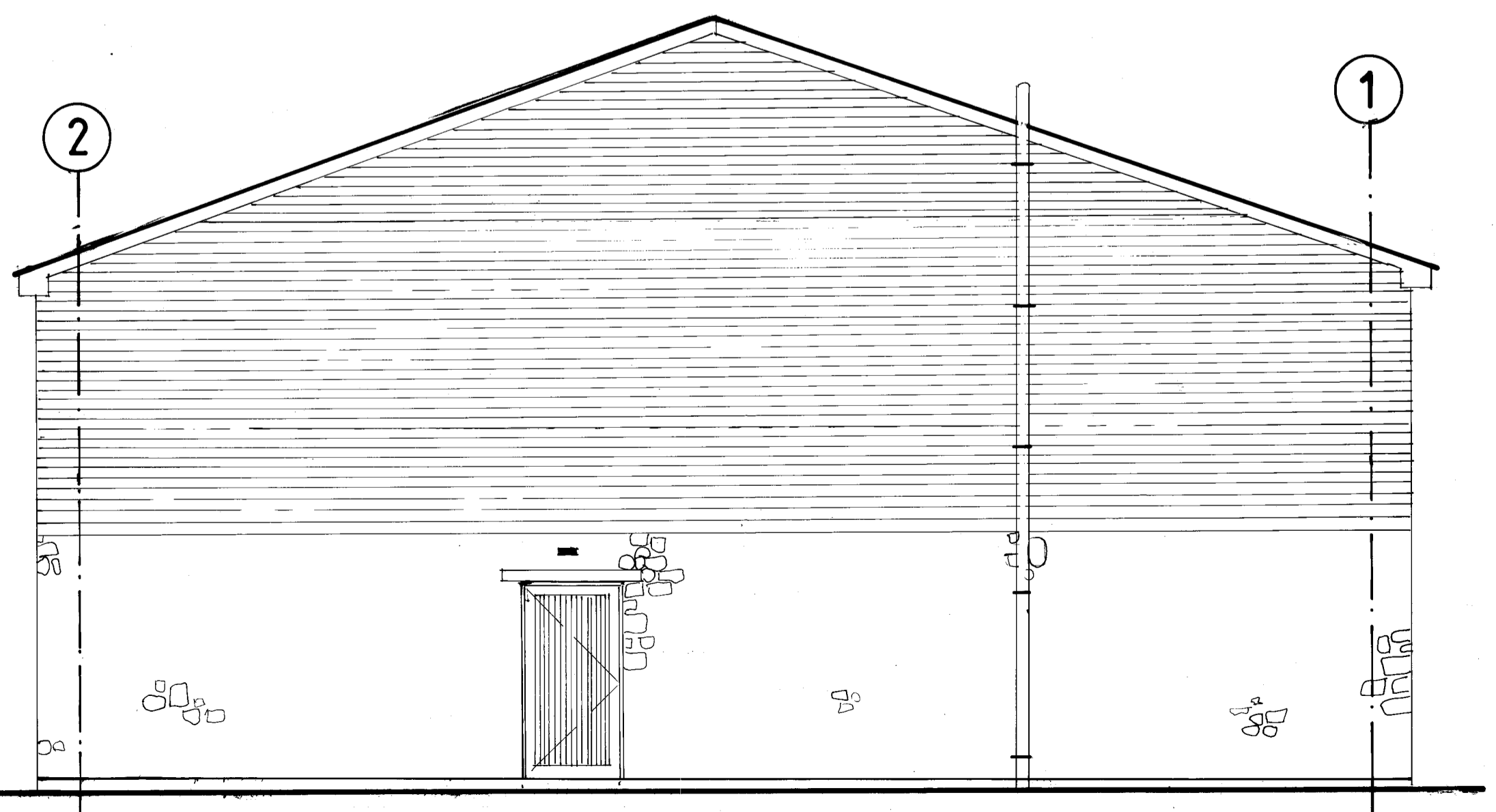
SOUTH ELEVATION
